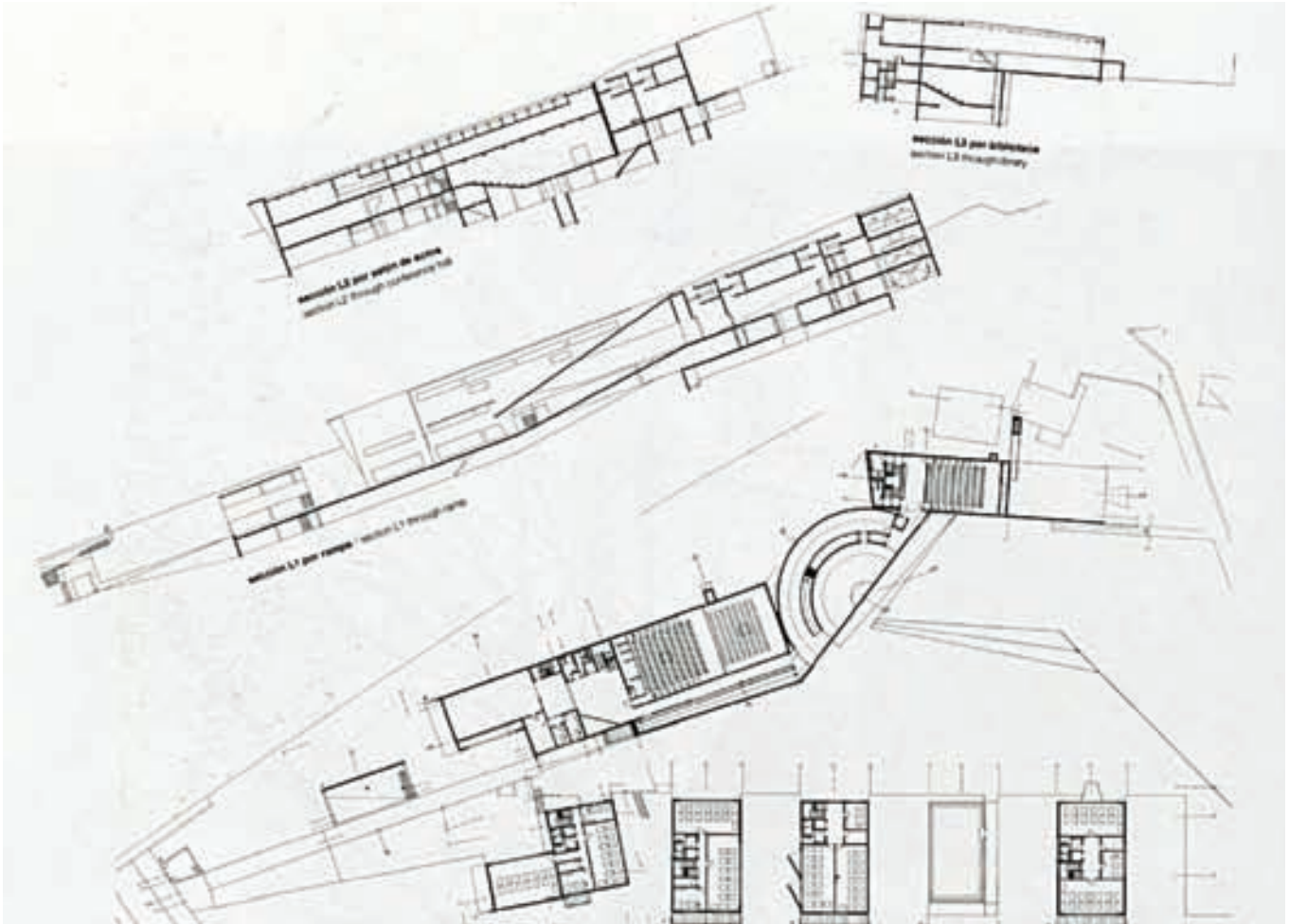
plan Rez+1
