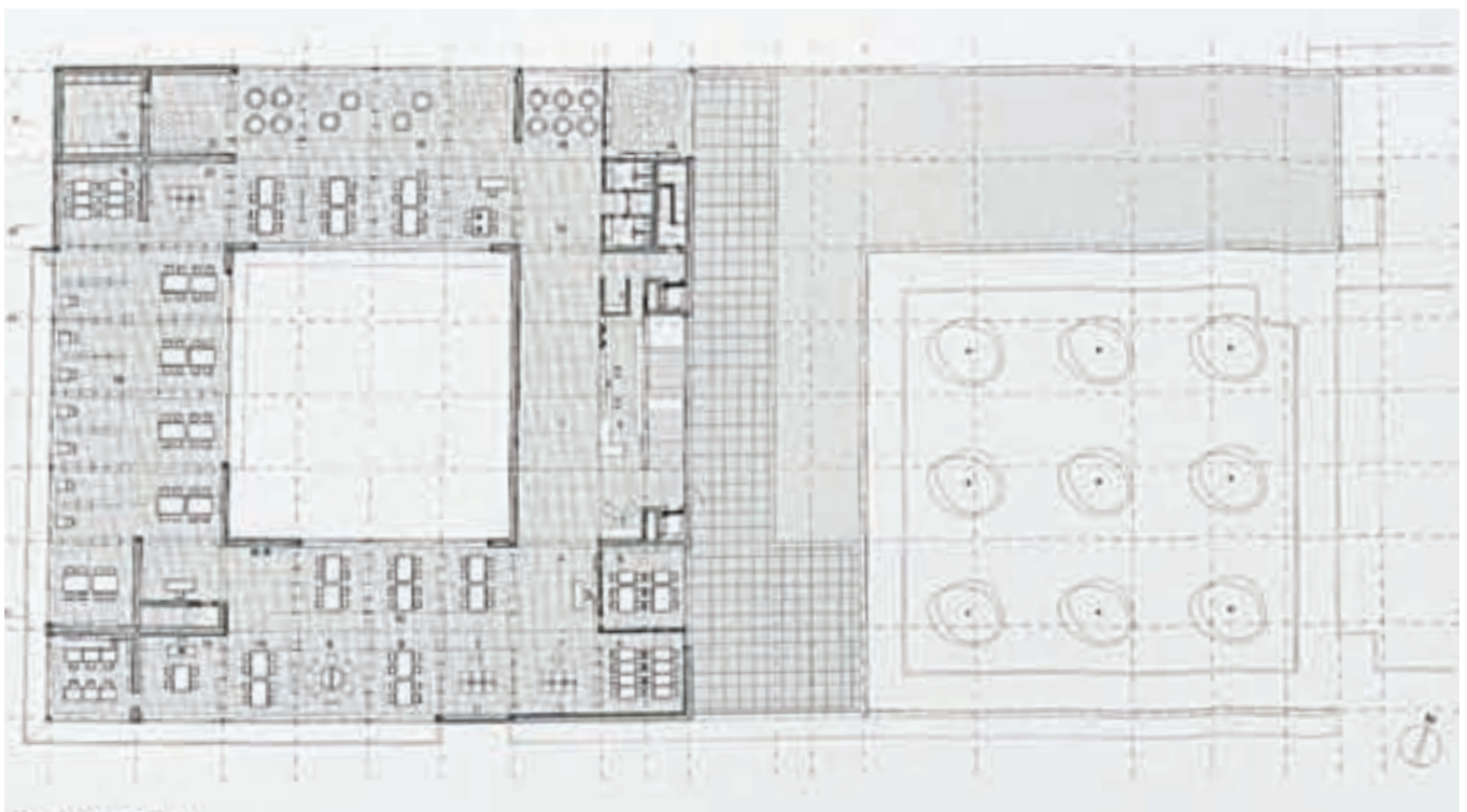
plan Rez+1
