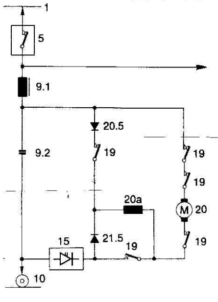
Montage BBC (traction)
