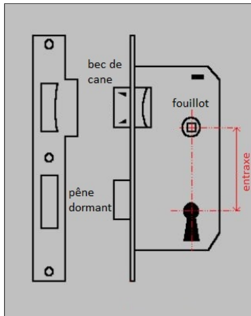
Figure 1: Schéma serrure
