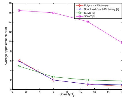
Fig. 3. Comparison of the polynomial dictionary with the SGWT, K-SVD and the graph structured dictionary [4] in terms of approximation performance in the Flickr dataset.
