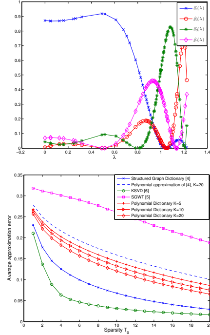
Fig. 1. (a) Learned kernels \{\widehat{g}_s(\cdot)\}_{s=1,2,3,4} with the polynomial dictionary algorithm. (b) Comparison of the polynomial dictionary with SGWT [5], K-SVD [6], the structured graph dictionary [4] and its polynomial approximation in terms of approximation performance in synthetic data.
