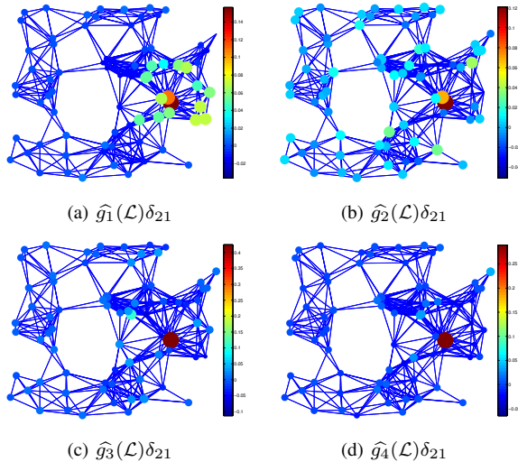
Fig. 2. Learned atoms centered on vertex n = 21 , from each of the subdictionaries.
