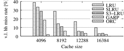
Fig. 3: Missed very large heavy-hitters vs. cache size (Mawi trace).
